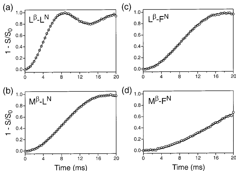
Figure 9. Representative internuclear distance measurements in N -formyl-[U- 13 C, 15 N]L-Met-L-Leu-L-Phe. Experimental \Delta S/S_0 curves (○) and analytical simulations (—) are shown for the selective pairwise recoupling of (a) Leu(C β )-Leu(N), (b) Met(C β )-Leu(N), (c) Leu(C β )-Phe(N), and (d) Met(C β )-Phe(N). The experiments shown have been performed on [U- 13 C, 15 N]MLF undiluted in natural abundance material, but are not appreciably affected by intermolecular couplings (see Supporting Information). Experiments were performed at \omega_r/2\pi = 10.0 kHz \pm 5 Hz, and 32 scans were averaged for each time point. The 13 C Gaussian pulse was 2.0 ms for experiments involving Met(C β ) and Leu(C β ), and 4.0 ms for Met(C γ ) and Leu(C γ ). The Met(C β )/Leu(C β ) distance measurements were performed simultaneously. The 15 N Gaussian pulse was 10.0 ms, applied on resonance with Met(N), Leu(N) or Phe(N). The summary of all distance measurements in N -formyl-[U- 13 C, 15 N]L-Met-L-Leu-L-Phe is given in Table 3.
